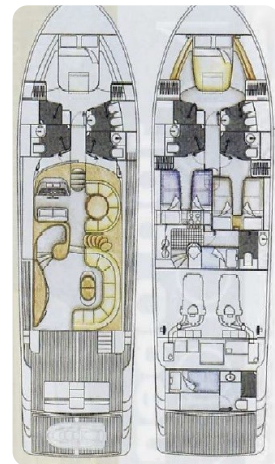
Uniesse 55 MY layout
