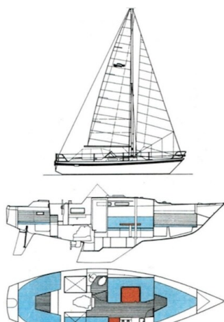
Targa-96-drawing
