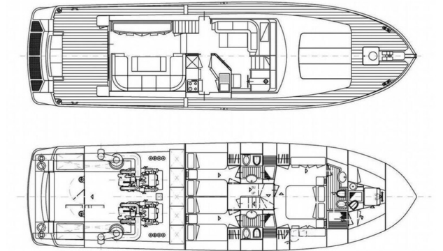
SANLORENZO SL 62 layout
