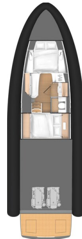
Strider15-Lower-Deck
