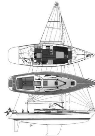
nordborg_40_drawing
