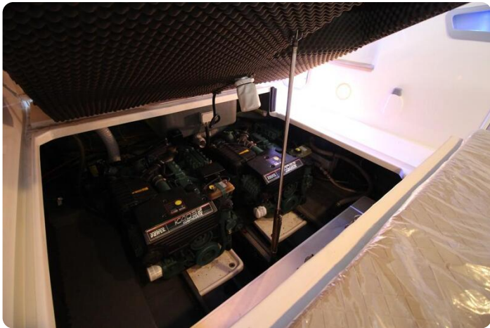
Airon Marine 325
